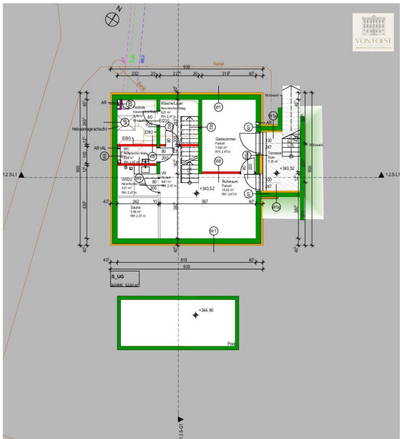
Grundriss 1.2.S-UG
