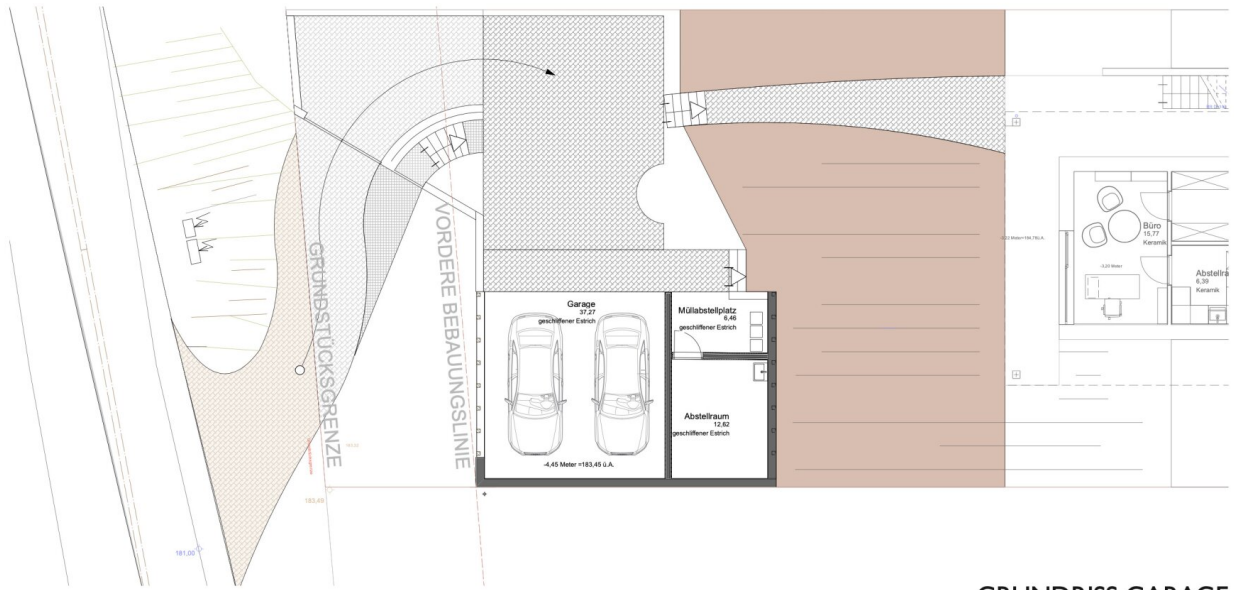
GRUNDRISS GARAGE
