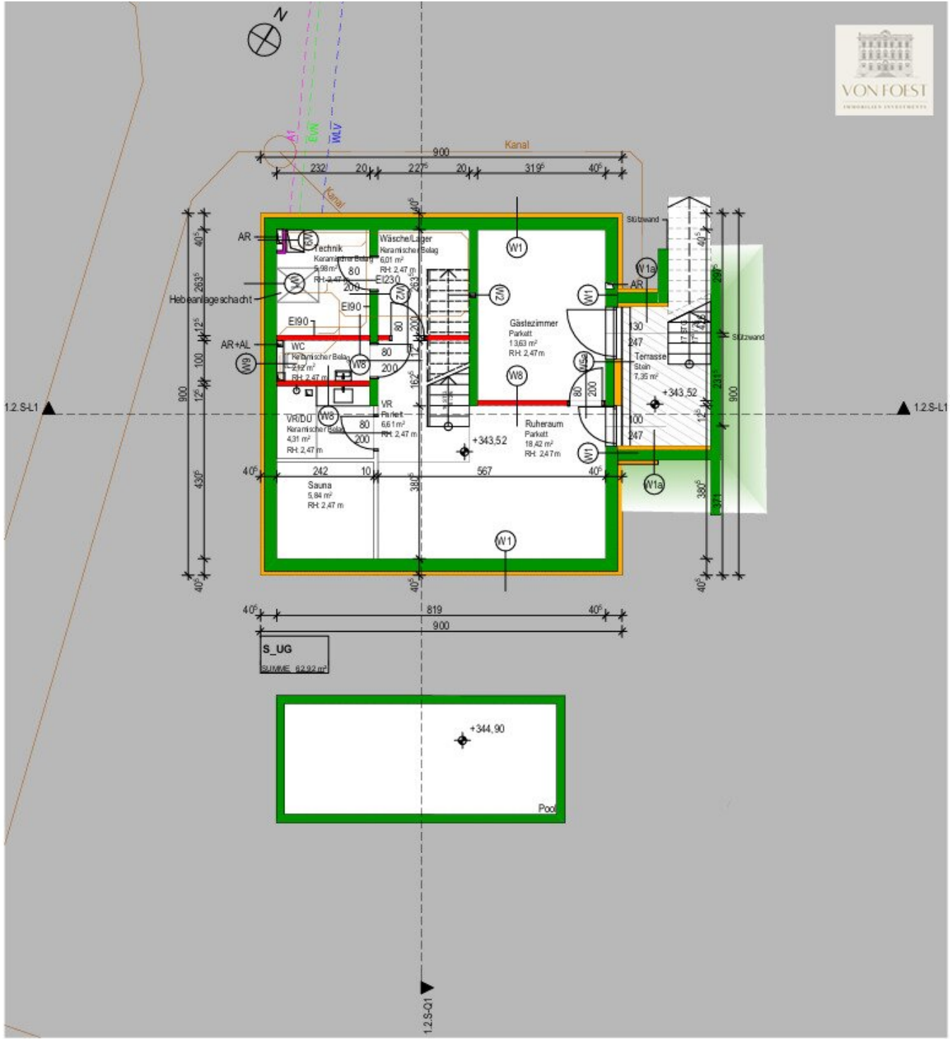
Grundriss 1.2.S-UG
