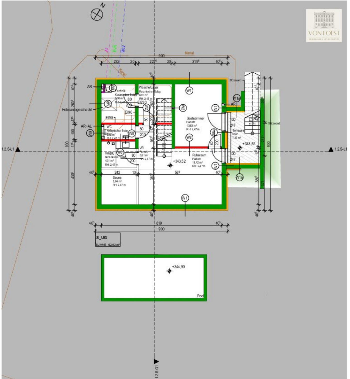
Grundriss 1.2.S-UG
