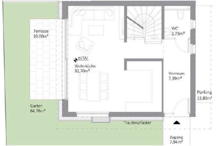
ERDGESCHOSS WNF 42,84m 2
